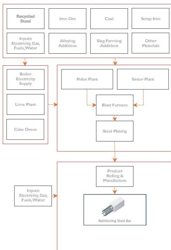
Integrated Iron & Steelmaking Production Route for Rebar
